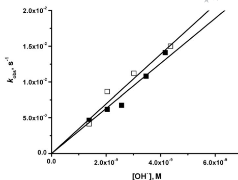
Figure 7. The dependence of the pseudo-first-order rate constant k_{f,\text{obs}} on [OH - ] concentration for formation of EuL 1 (□) and EuL 2 (■).
